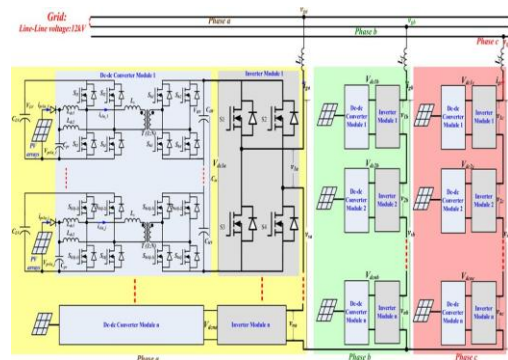
fig. 1 Proposed grid-connected PV system with cascaded multilevel converters at 3 MW.
