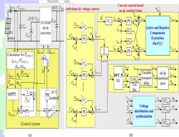
Fig. 2 Proposed control system of the grid-connected cascaded PV converters in phase a. (a) CF-DAB dc-dc converters control of one unit in module 1. (b) Cascaded multilevel inverters control.
