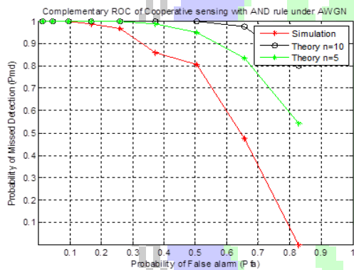
Fig 7: Spectrum sensing with AND rule The PM (increased detection performance) rapidly improves with increasing average SNR.
