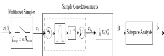
Figure 3. Proposed wideband spectrum sensing model.
