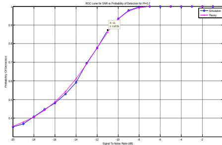
Fig 6:Probability of Detection Vs SNR
