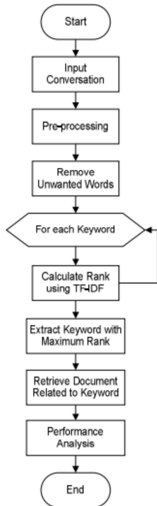
Figure 2: Flowchart of Proposed architecture
