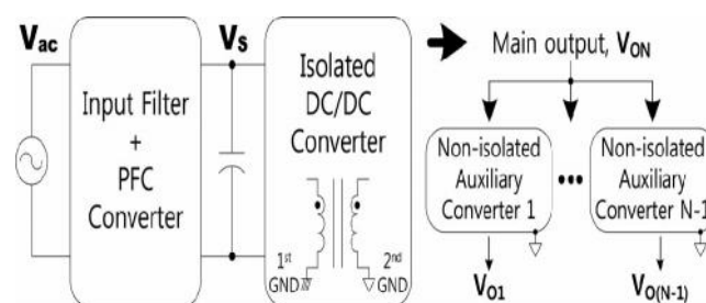
Fig 1. Block diagram of N multioutput power supply with nonisolated auxiliary converter
