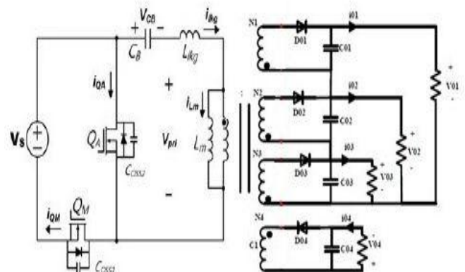
Fig 3. Block diagram of proposed Multi output Fly back converter
