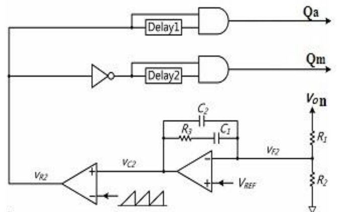
Fig 5. Gate signals
