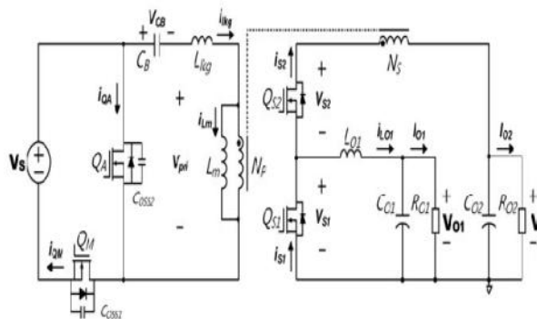
Fig 2. Conventional Fly back converter with two outputs
