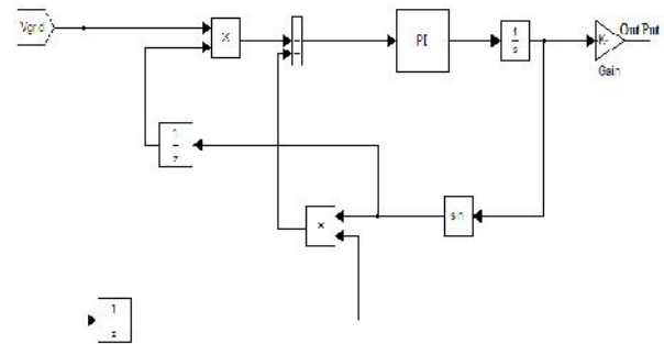
Fig.3 Block scheme of the delay-based PLL.
