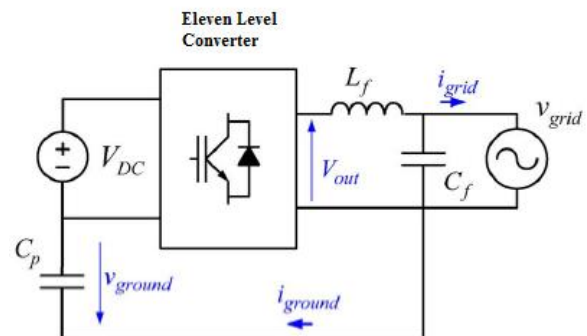
Fig. 4. Schematic of the test bed employed for the experiments.
