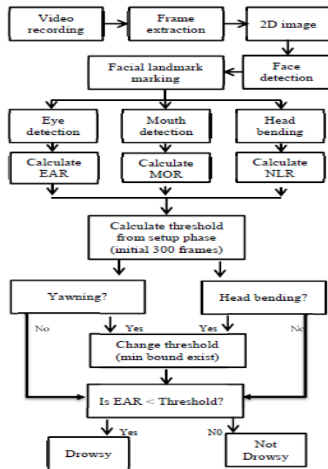
Fig. 1 The block diagram of the proposed drowsiness detection system
