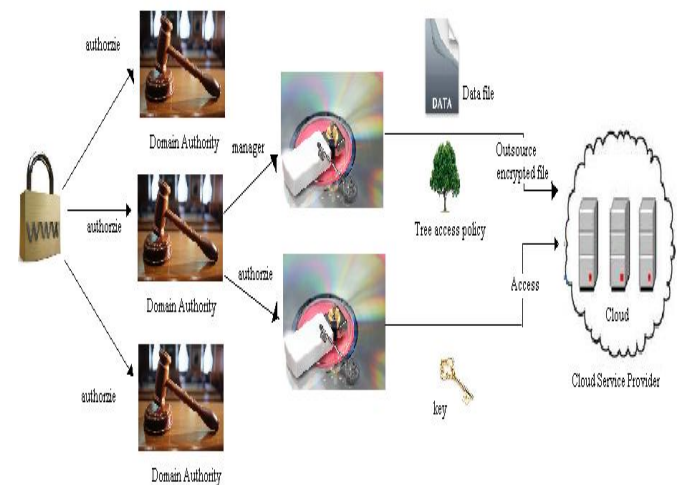
Fig.2. System Model
