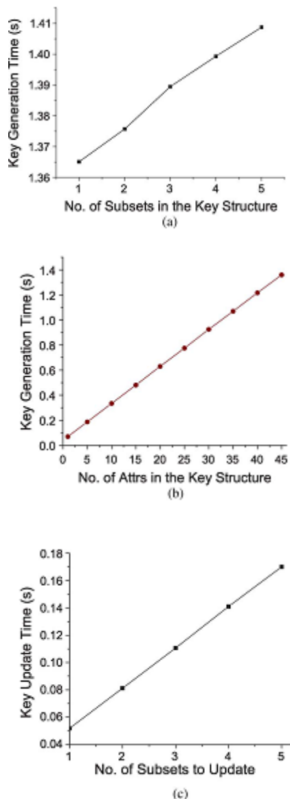
Fig.3. Experiments on new user/domain authority grant and key update. (a) New user/domain authority grant (b) user/domain authority grant (c) key update
