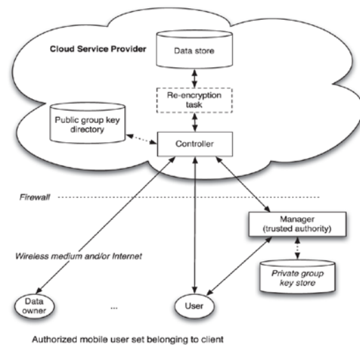
Figure 1: Cloud data storage with respect to cryptography.
