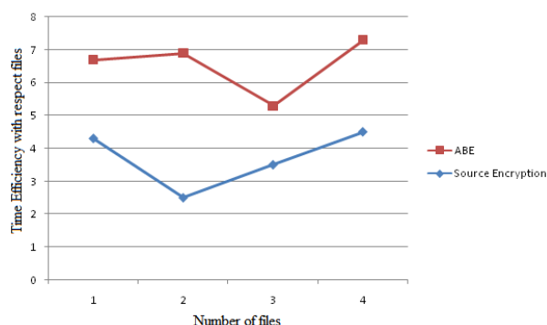
Figure 4: Comparison analysis for access files with respect to time.
