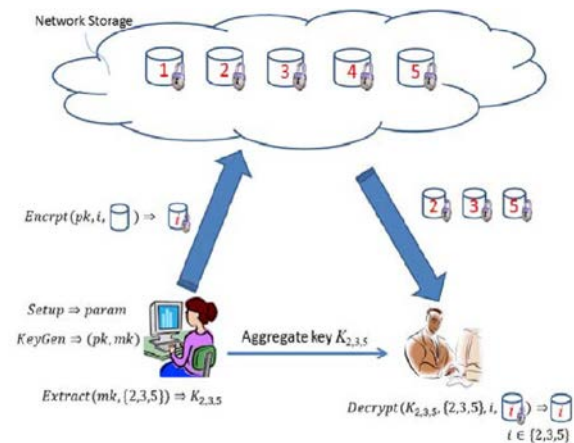
Figure 2: Key aggregate system for outsourcing data in cloud.
