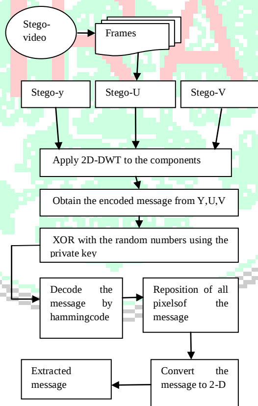
Fig 5: Block diagram for data extracting phase
