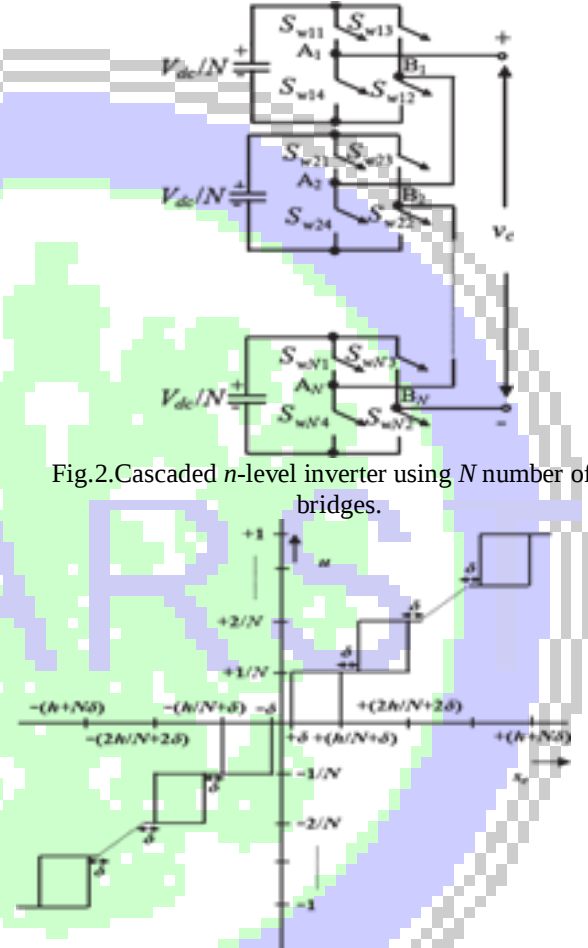
Fig. 3.Multiband hysteresis modulation.
