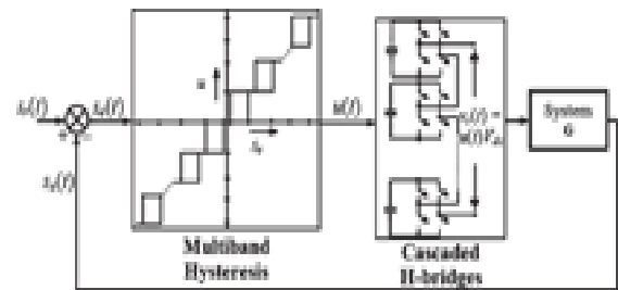
Fig. 4 Block diagram for a generalized n -level inverter-controlled system using multiband hysteresis modulation
