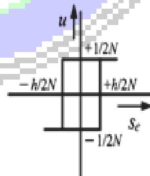
Fig. 6. Switching characterization of an n -level inverter using the PTH hysteresis band.
