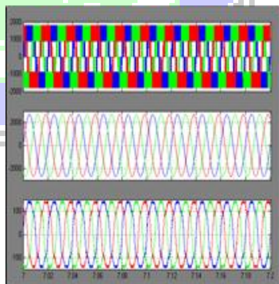
Fig.10 Three phase inverter voltage, Source voltage and source current Fig.10 shows the three phase inverter output voltage, source voltage and current which are not having harmonics.
