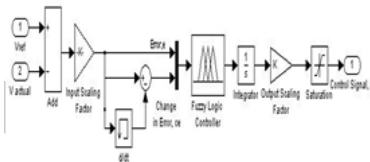
Fig 9: SIMULINK model of proposed FLC.
