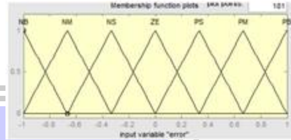
Fig.7.Membership functions
