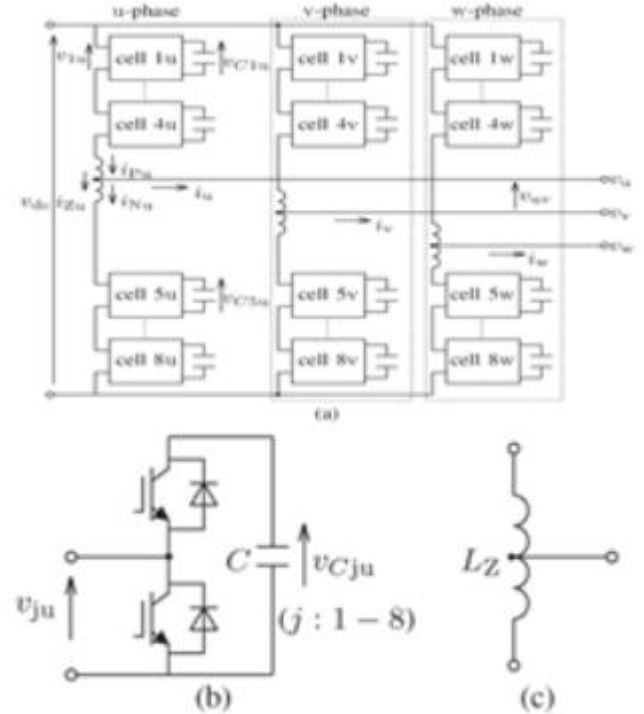
Fig.1. Circuit configuration for an MMCI-DSCC. (a) Power circuit. (b) Chopper cell. (c) Center-tapped inductor.
