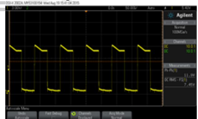
Figure 14: Pulses to S_a
